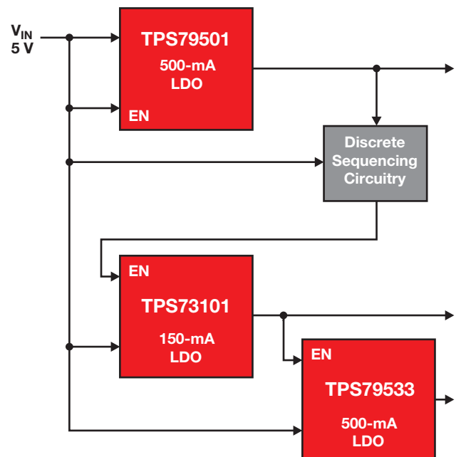
LDO power solution.
