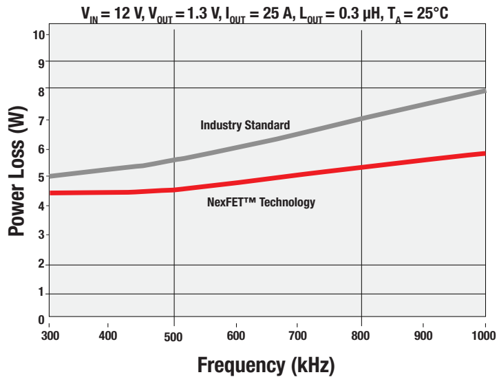
Same power loss, double the frequency.
