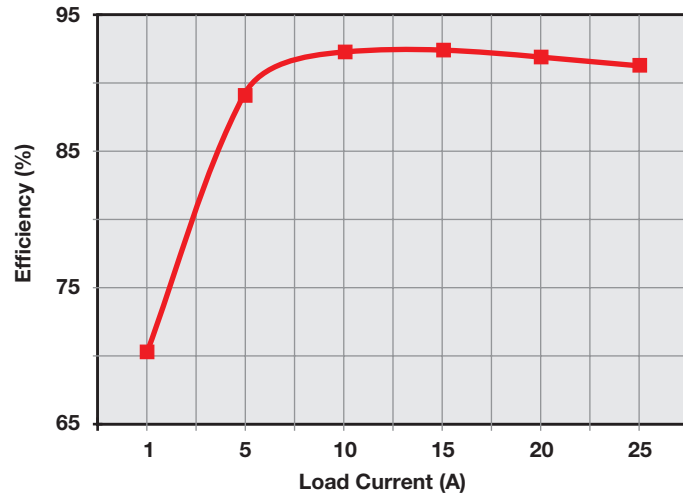
Typical UCC28230 efficiency plot.
