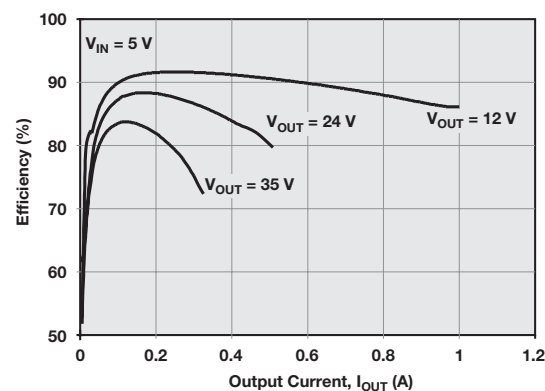
TPS61175 efficiency.
