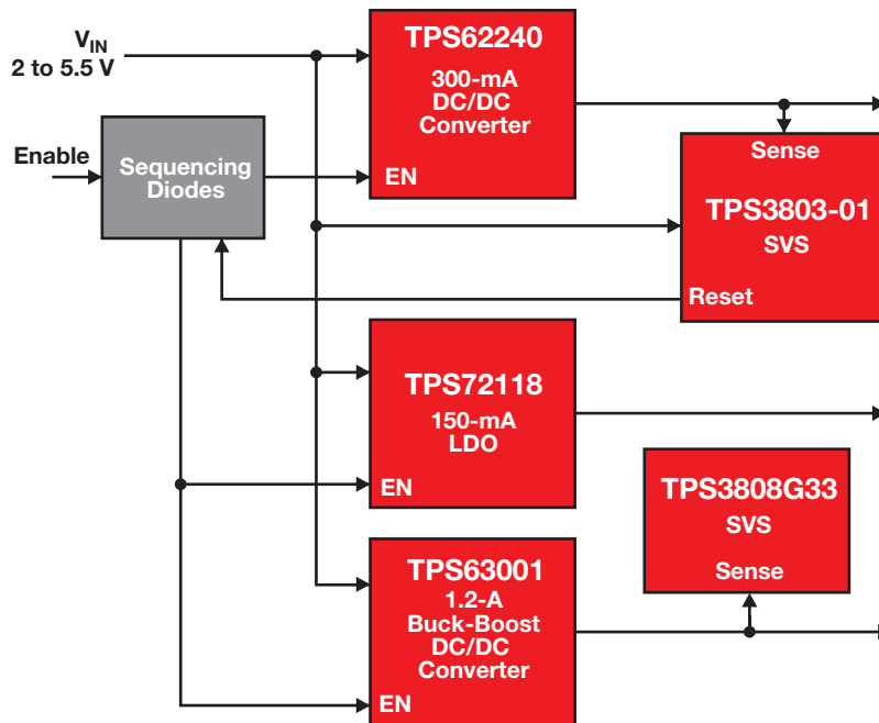
Wide V_{IN} , high-efficiency, discrete power solution.
