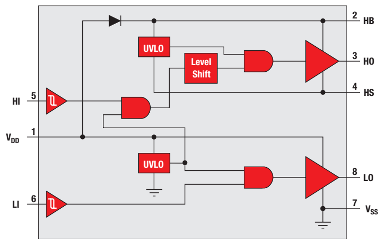
UCC27200/01 block diagram.
