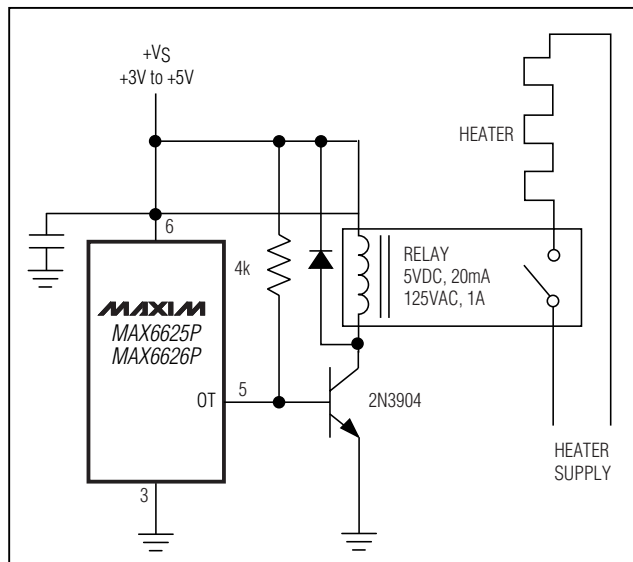
Figure 8. Simple Thermostat
