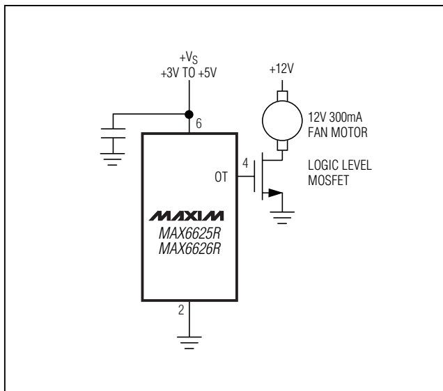
Figure 7. Fan Controller
