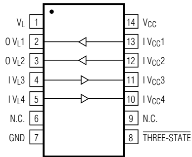
TSSOP-14
