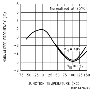
Oscillator Frequency
