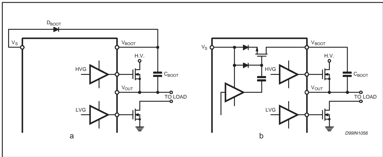
Figure 3. Bootstrap Driver.
