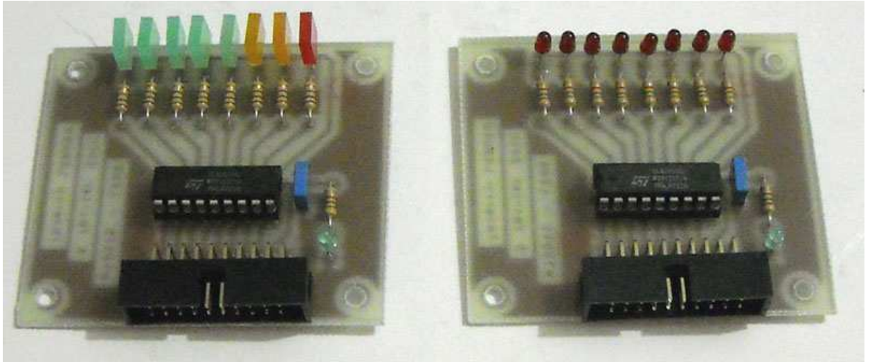
Figure 5.5 Interface 8 LEDs (images-maquettes\AT8535-LED8-12.jpg).
