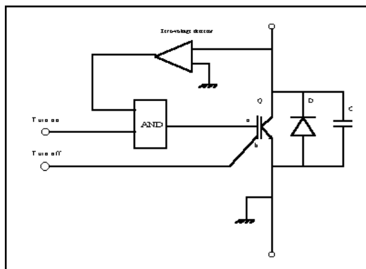
Figure 2 Functional diagram of Thyristor-dual
