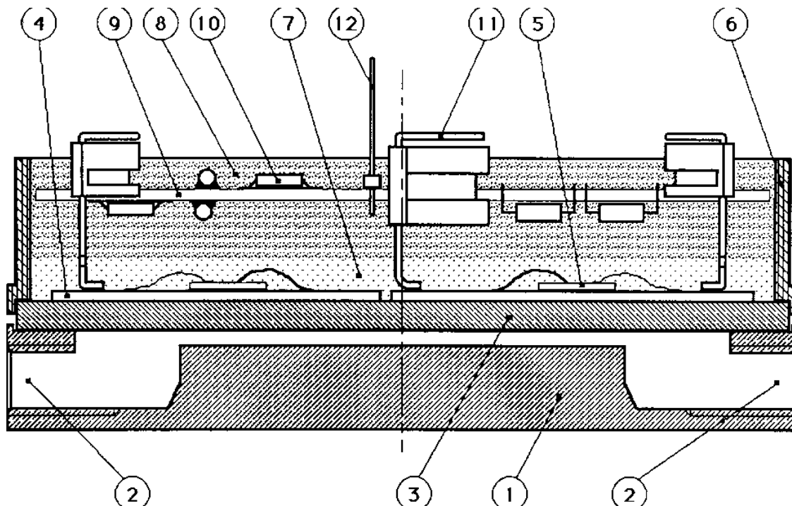
Figure 5 Integral Liquid Cooled Module
