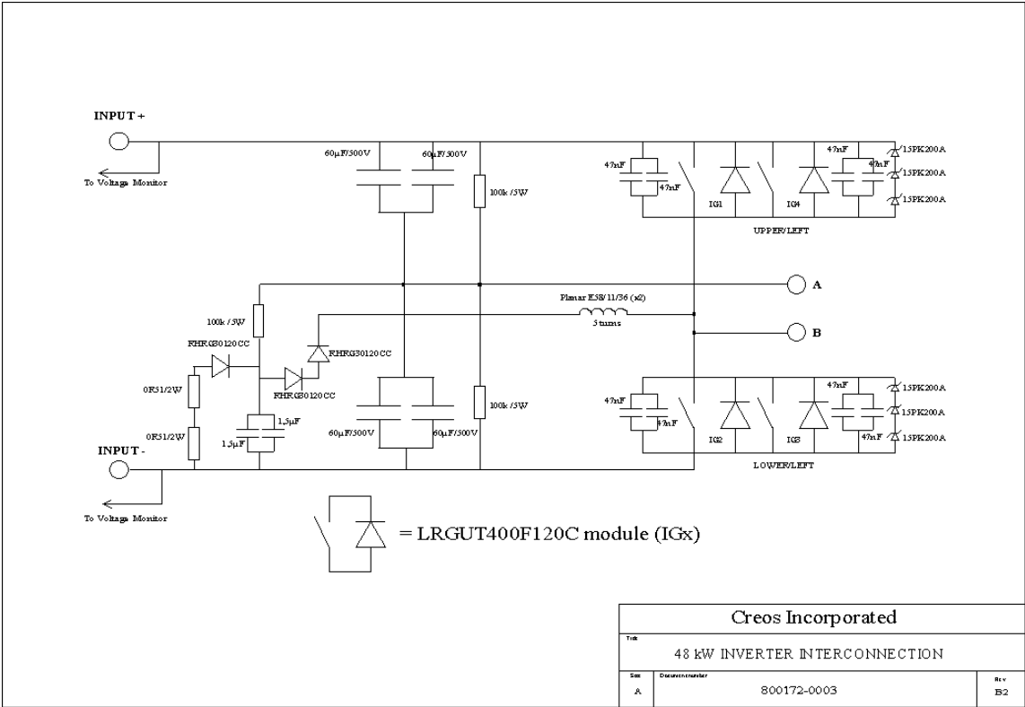
Figure 1 Inverter interconnections
