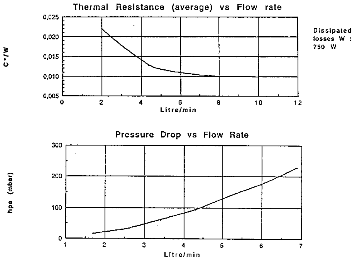
Figure 6 MU20M4-ILC Thermal Performance
