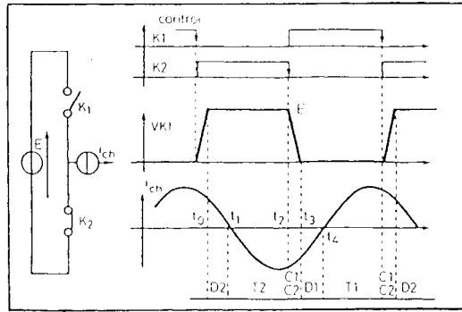
Figure 3 Waveforms and control signals
