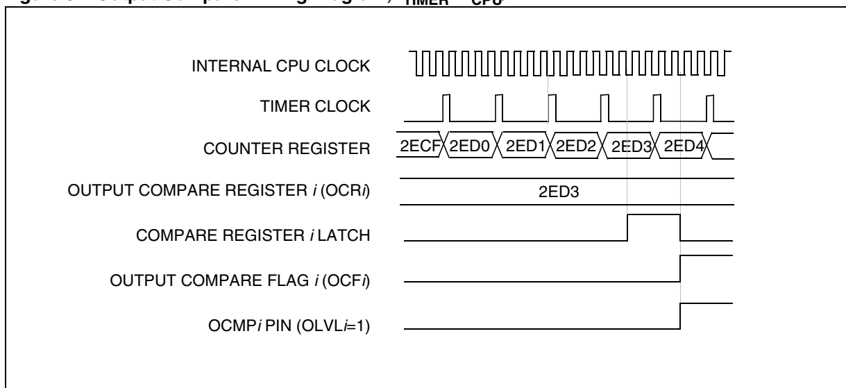
Figure 52. Output Compare Timing Diagram, f_{\text{TIMER}} = f_{\text{CPU}}/4
