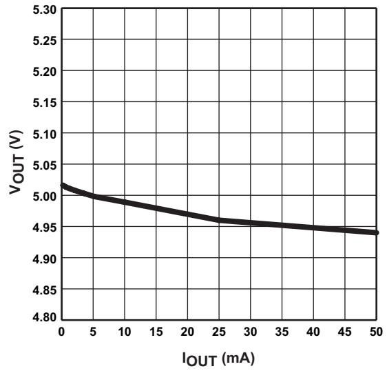
Load Regulation
