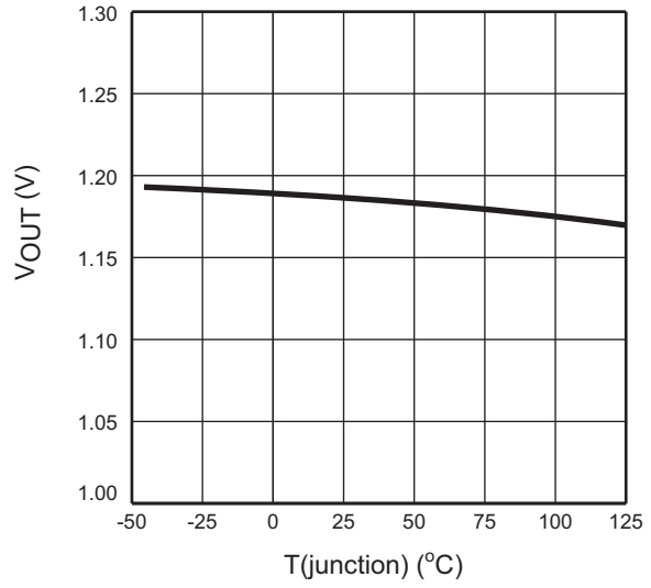
Temperature Variation
