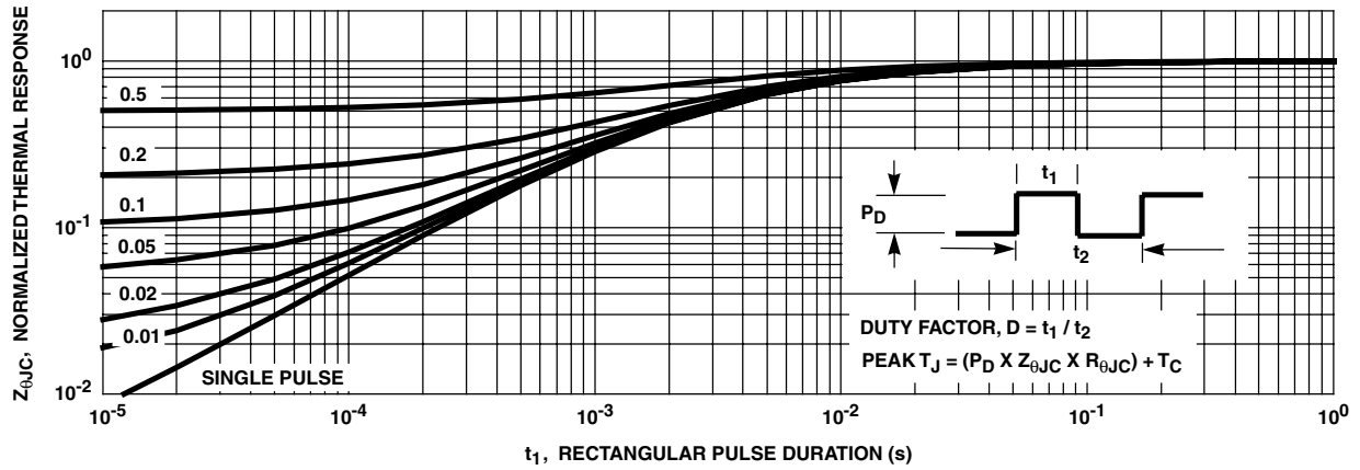
FIGURE 17. NORMALIZED TRANSIENT THERMAL RESPONSE, JUNCTION TO CASE
